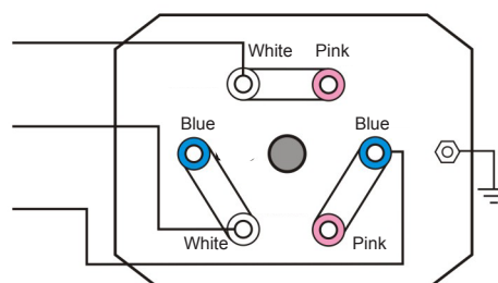
Heating element connected for 220-240V 3-phase
