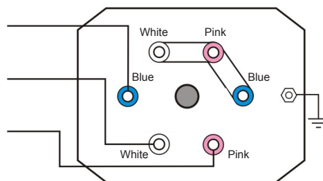
Heating element connected for 380-415V 3-phase
